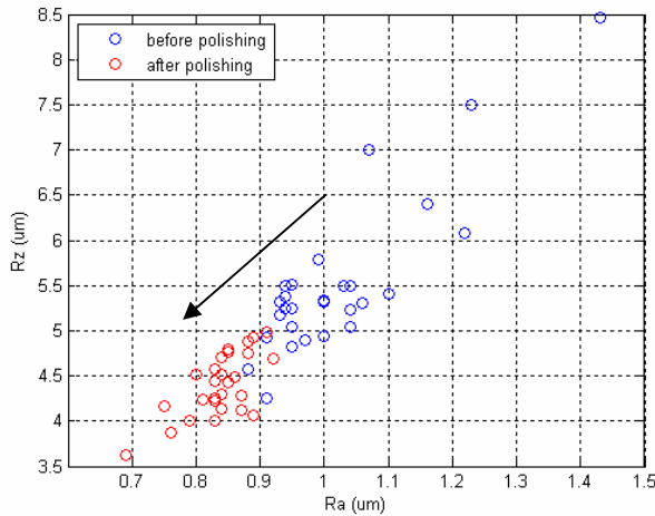
Figure 5. The changing of surface roughness value before and after polishing
