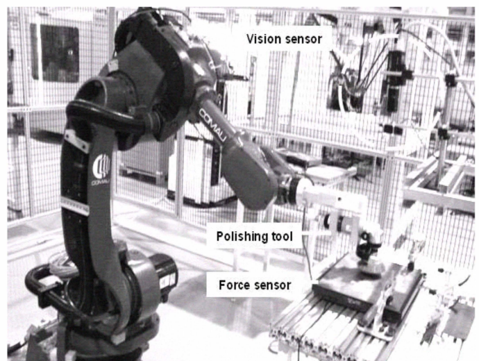
Figure 1. Implementation of the polishing robot system
