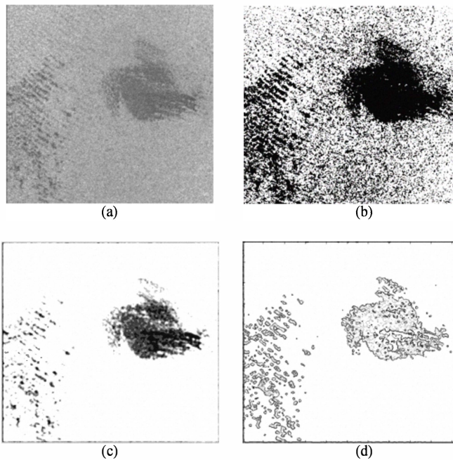
Figure 2. Surface defect characterization on corrosion image: (a) Original image taken from vision system; (b) Threshold image with non-uniform noise; (c) Filtering image with Gaussian filter; (d) Feature in two level defect.
