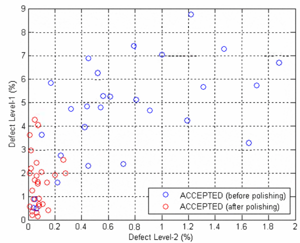
Figure 4. The changing of defect levels before and after polishing
